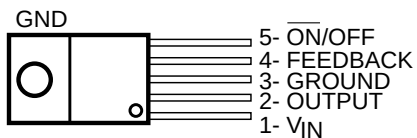
5-LEAD TO-220 (T)
