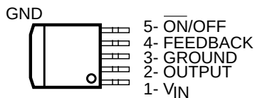
5-LEAD TO-263 (U)
