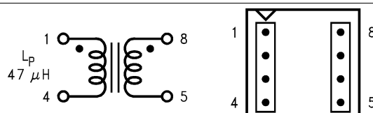
Figure 35. Pulse Pe-68414 (Top View) (Surface Mount)
