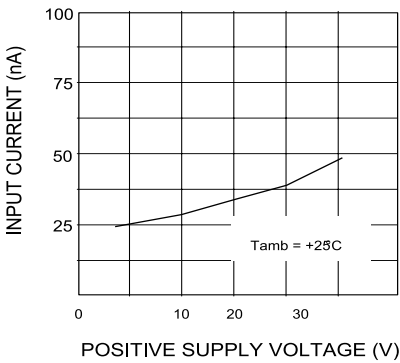
Figure 14: Input current
