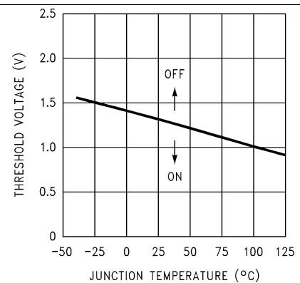
Figure 12. \overline{ON} /OFF Threshold Voltage
