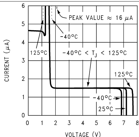
Figure 14. Shutdown/Soft-Start Current
