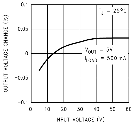
Figure 2. Line Regulation
