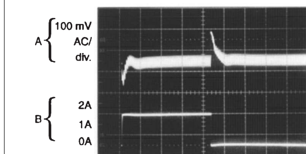
Figure 19. Continuous Mode Switching Waveforms
