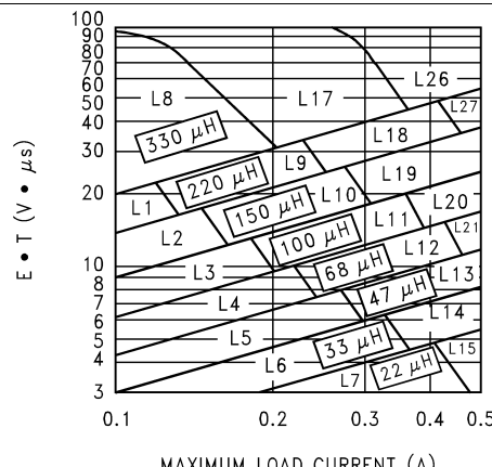
Figure 30. LM2594xx Adjustable Voltage
