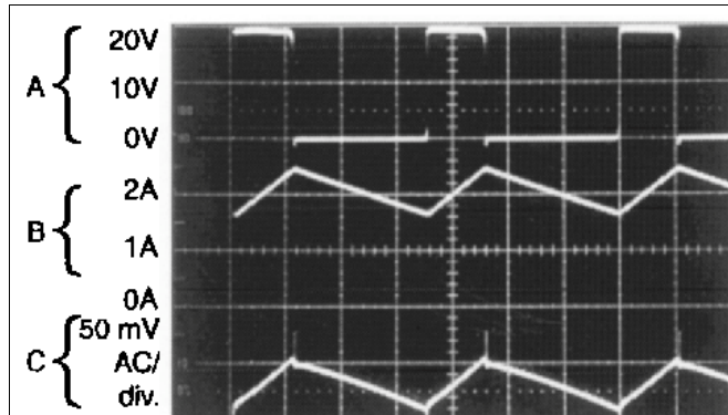
Continuous Mode Switching Waveforms V_{IN} = 20\text{ V} , V_{OUT} = 5\text{ V} , I_{LOAD} = 2\text{ A} , L = 32\text{ } \mu\text{H} , C_{OUT} = 220\text{ } \mu\text{F} , C_{OUT}\text{ ESR} = 50\text{ m}\Omega A: Output Pin Voltage, 10 V/div. B: Inductor Current 1 A/div. C: Output Ripple Voltage, 50 mV/div.
