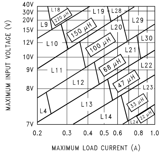
Figure 36. LM2598-5.0
