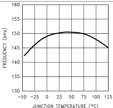
Figure 12. Switching Frequency
