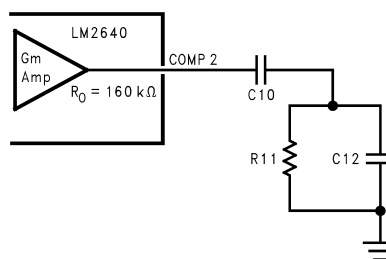
Figure 21. Typical Compensation Network
