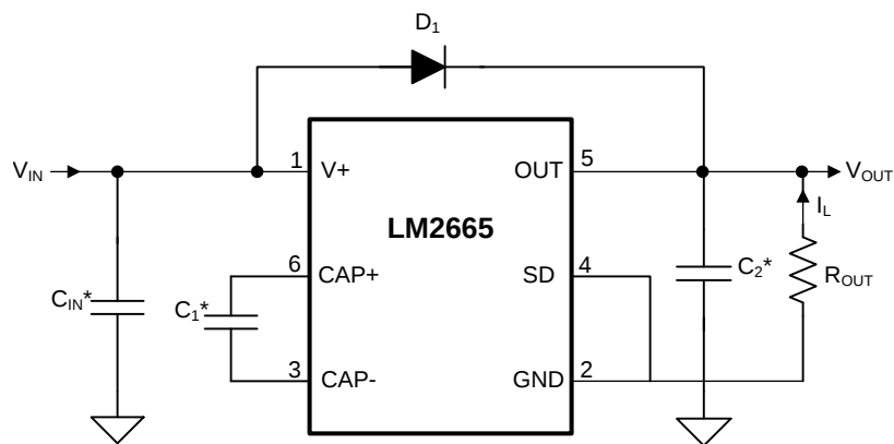
Figure 9. LM2665 Test Circuit
