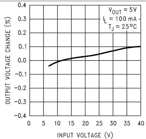
Figure 2. Line Regulation
