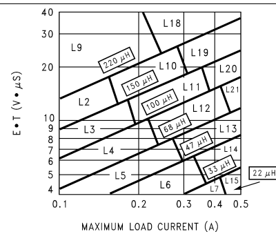
Figure 27. LM2674, Adjustable Version
