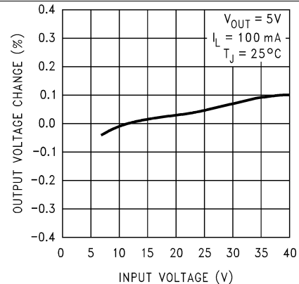
Figure 2. Line Regulation
