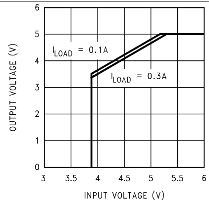
Figure 14. Dropout Voltage, 5-V Version
