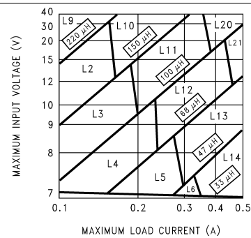
Figure 25. LM2674, 5-V Version
