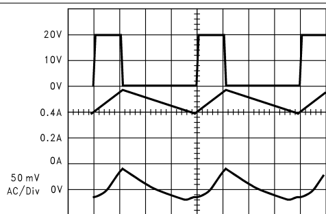
Continuous mode switching waveforms V_{IN} = 20 V, V_{OUT} = 5 V, I_{LOAD} = 500 mA L = 100 \mu H, C_{OUT} = 100 \mu F, C_{OUT}ESR = 0.1 \Omega A: V_{SW} pin voltage = 10 V/div B: Inductor current = 0.2 A/div C: Output ripple voltage = 50 mV/div ac-coupled
