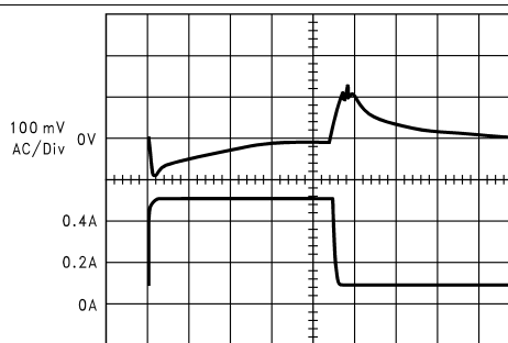
Load transient response for continuous mode V_{IN} = 20 V, V_{OUT} = 5 V, L = 100 \mu H, C_{OUT} = 100 \mu F, C_{OUT}ESR = 0.1 \Omega A: Output voltage = 100 mV/div, ac-coupled B: Load current = 100-mA to 500-mA load pulse
