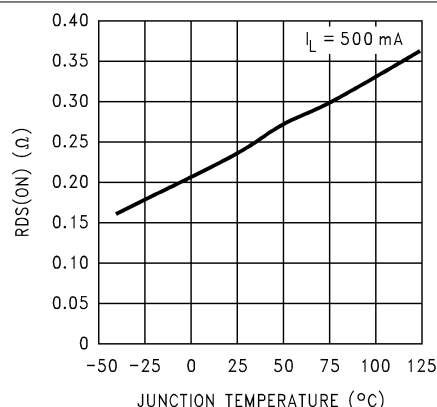
Figure 7-4. Drain-to-Source Resistance
