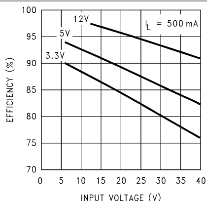
Figure 7-3. Efficiency
