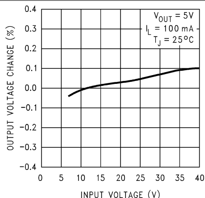
Figure 7-2. Line Regulation
