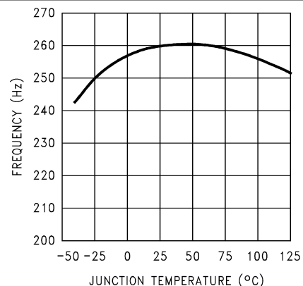
Figure 7-10. Switching Frequency
