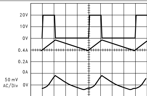
Continuous mode switching waveforms V_{IN} = 20 V, V_{OUT} = 5 V, I_{LOAD} = 500 mA L = 100 \mu H, C_{OUT} = 100 \mu F, C_{OUT}ESR = 0.1 \Omega A: V_{SW} pin voltage = 10 V/div B: Inductor current = 0.2 A/div C: Output ripple voltage = 50 mV/div ac-coupled
