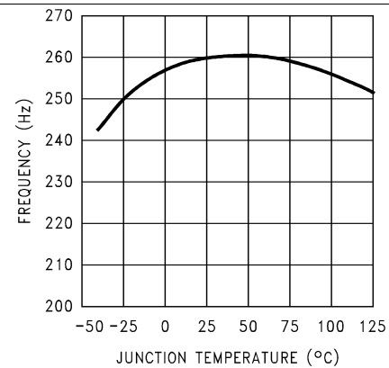
Figure 10. Switching Frequency
