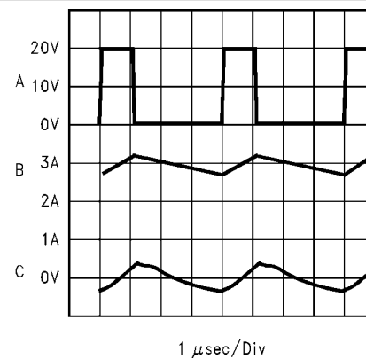
Figure 6-10. Switching Frequency
