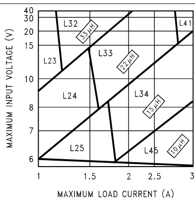
Figure 17. LM2676-3.3
