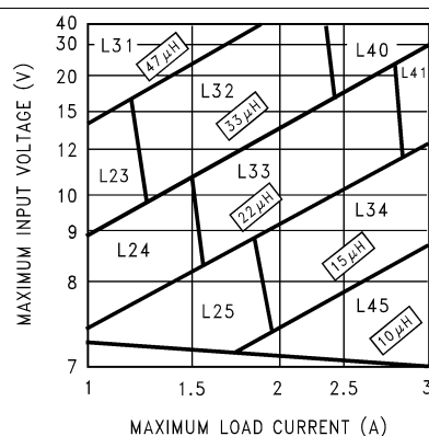
Figure 18. LM2676-5
