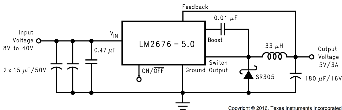
Figure 16. Basic Circuit for All Output Voltage Versions
