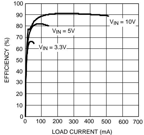
Figure 8. Efficiency vs Load Current ( V_{OUT} = 12\text{ V} )
