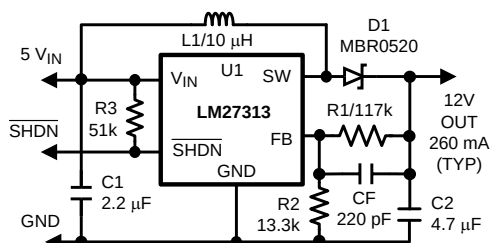
Figure 12. Typical Application Circuit
