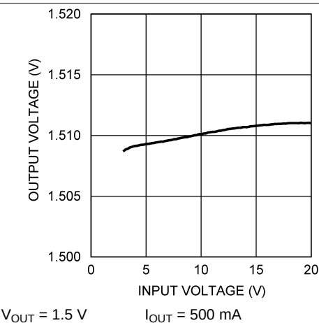
Figure 5. Line Regulation
