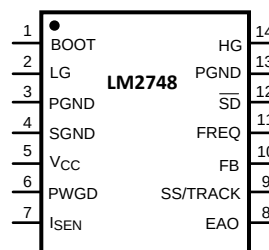
Figure 2. 14-Lead Plastic TSSOP, \theta_{JA} = 155^{\circ}\text{C/W} Top View Package Number PW0014A
