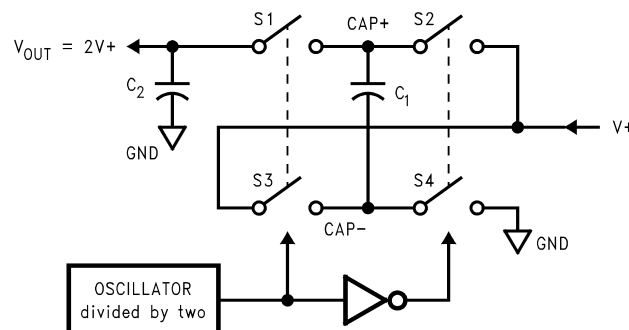
Figure 11. Voltage Doubling Principle
