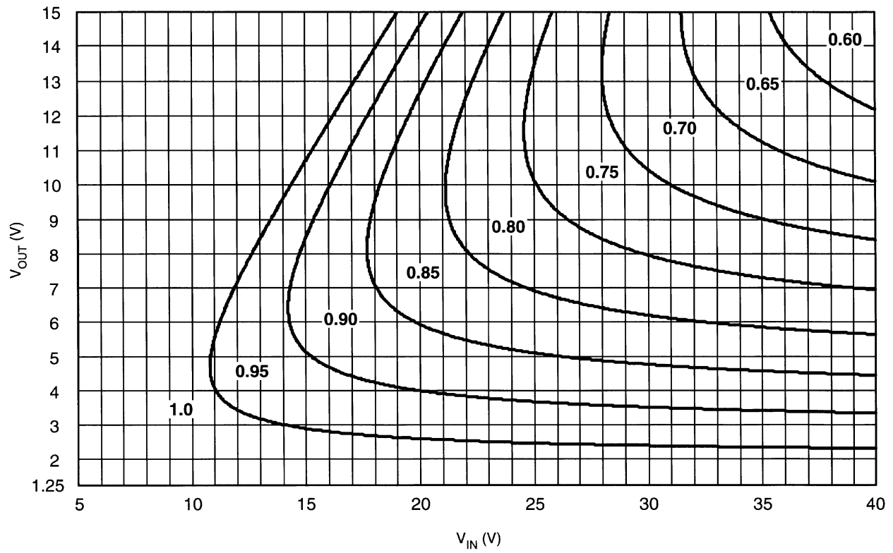
Figure 21. LM2825 Output Current Derating for T J = -25°C to 0°C
