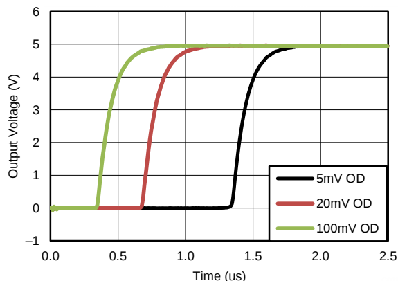
Figure 6. Response Time for Various Overdrives Positive Transition
