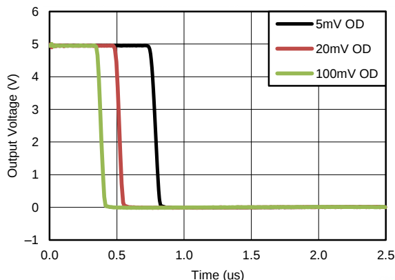
Figure 5. Response Time for Various Overdrives Negative Transition
