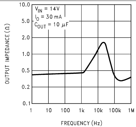
Figure 20. 5-V LM2936 Output Impedance
