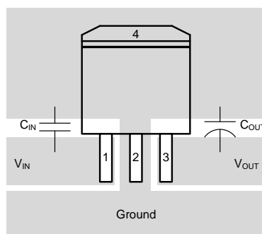
Figure 32. TO-263 Layout
