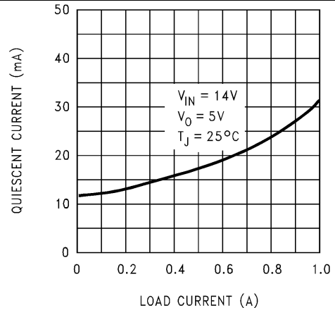
Figure 6. Quiescent Current
