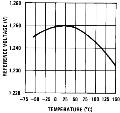
Figure 7. Temperature Stability
