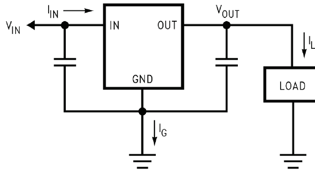
Figure 38. Power Dissipation Diagram
