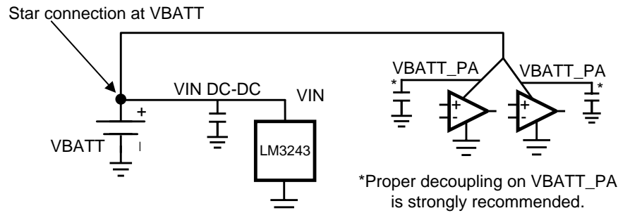
Figure 26. VBATT Star Connection on VIN And VBATT_PA
