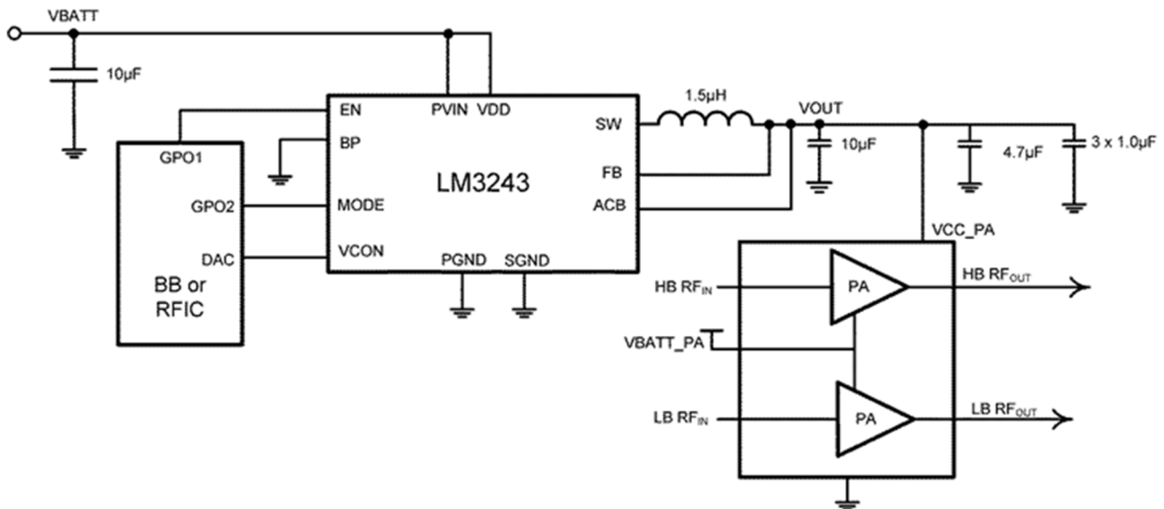
Figure 27. Simplified LM3243 RF Evaluation Board Schematic
