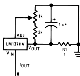
Figure 8. Current Regulator
