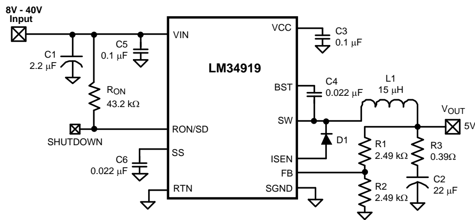
Figure 15. Example Circuit
