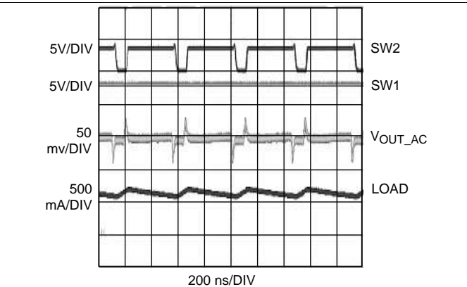
Figure 36. Typical Switching Waveform in Boost Mode (PWM Mode) V_{IN} = 3\text{ V} , V_{OUT} = 3.4\text{ V} , Load = 500 mA
