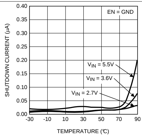
Figure 2. Shutdown Current vs Temp
