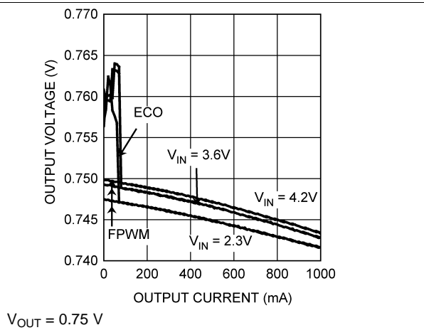
Figure 7. Output Voltage vs Output Current
