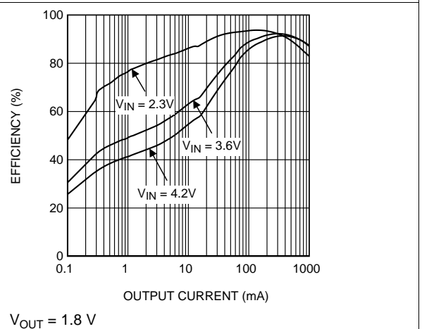
Figure 12. Efficiency vs Output Current, ECO Mode
