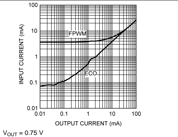
Figure 9. Input Current vs Output Current
