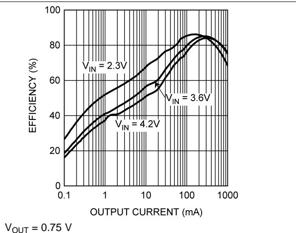
Figure 11. Efficiency vs, Output Current, ECO Mode
