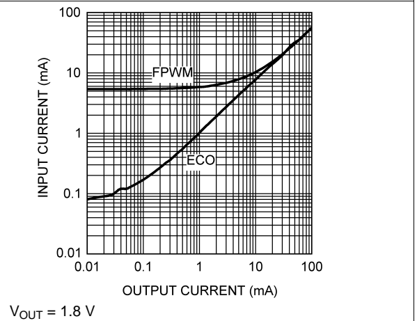
Figure 10. Input Current vs Output Current
