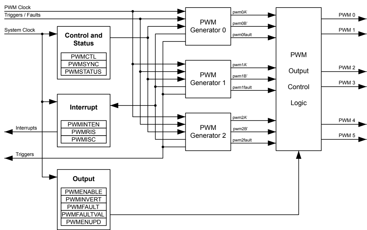
Figure 18-1. PWM Module Diagram
