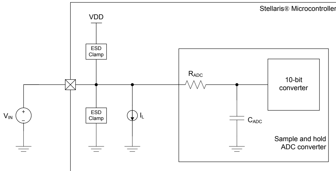
Figure 20-14. ADC Input Equivalency Diagram
