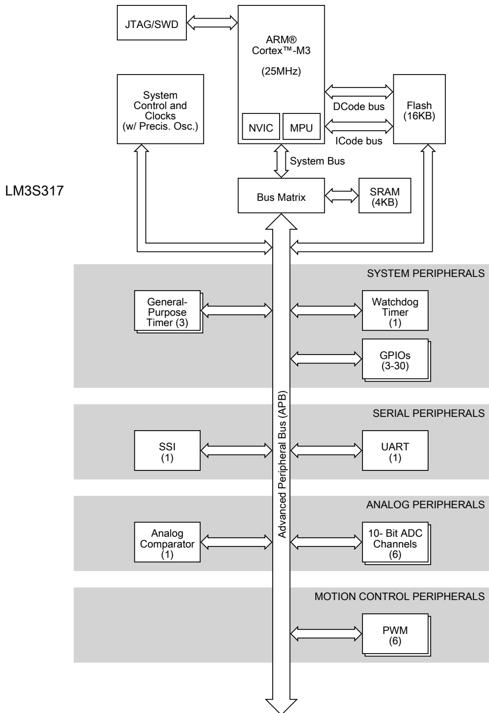
Figure 1-1. Stellaris LM3S317 Microcontroller High-Level Block Diagram
