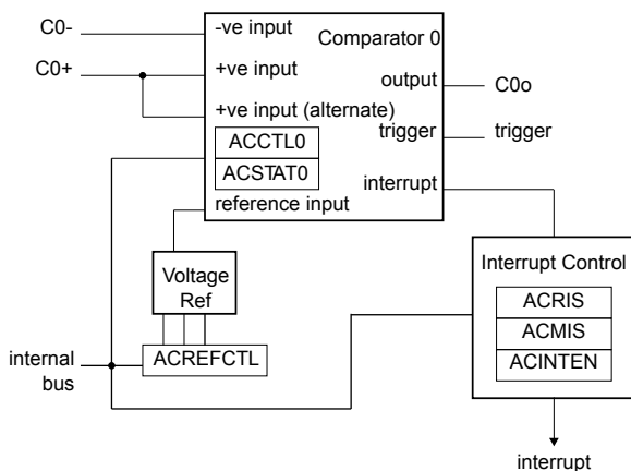
Figure 13-1. Analog Comparator Module Block Diagram
