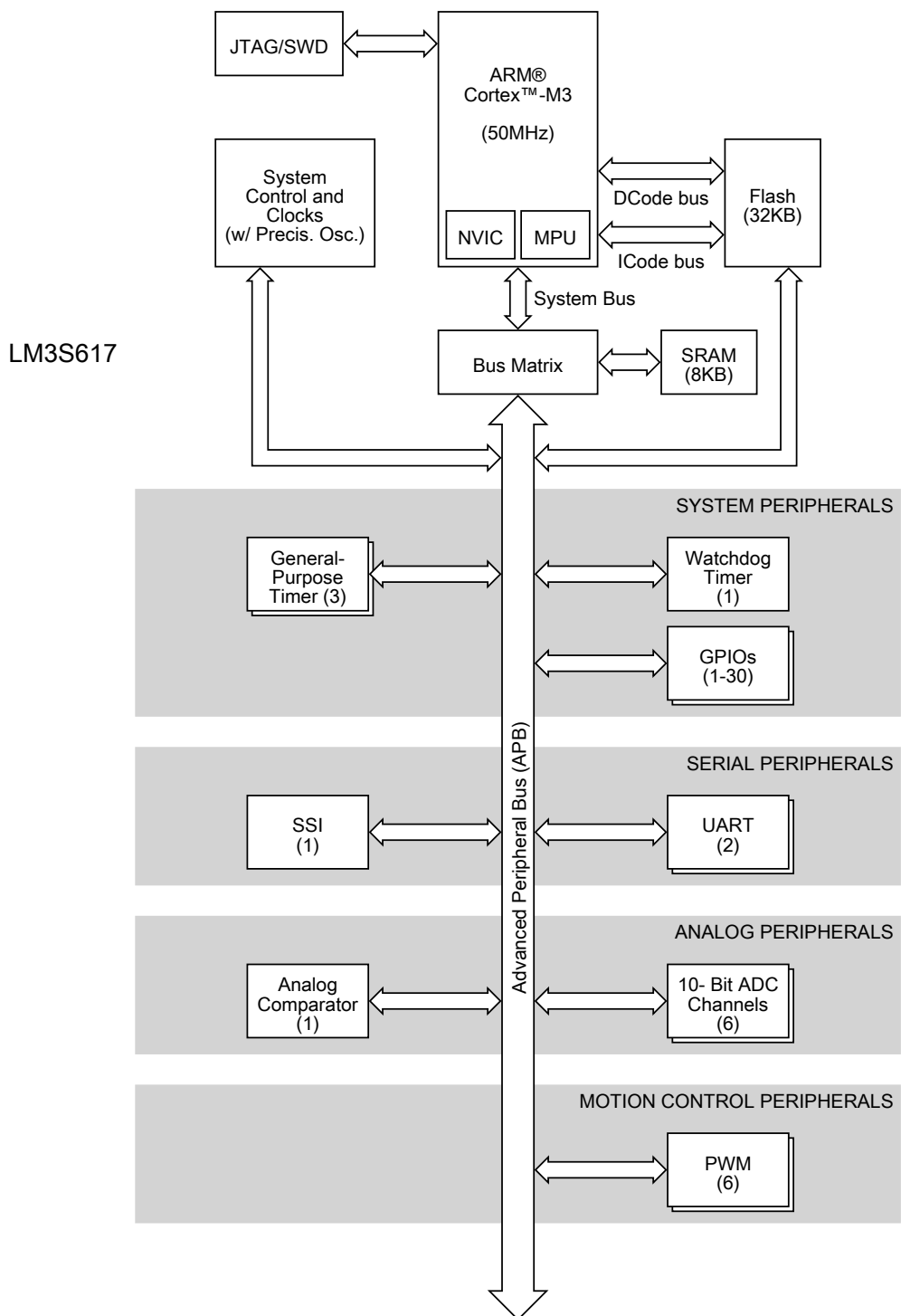
Figure 1-1. Stellaris LM3S617 Microcontroller High-Level Block Diagram
