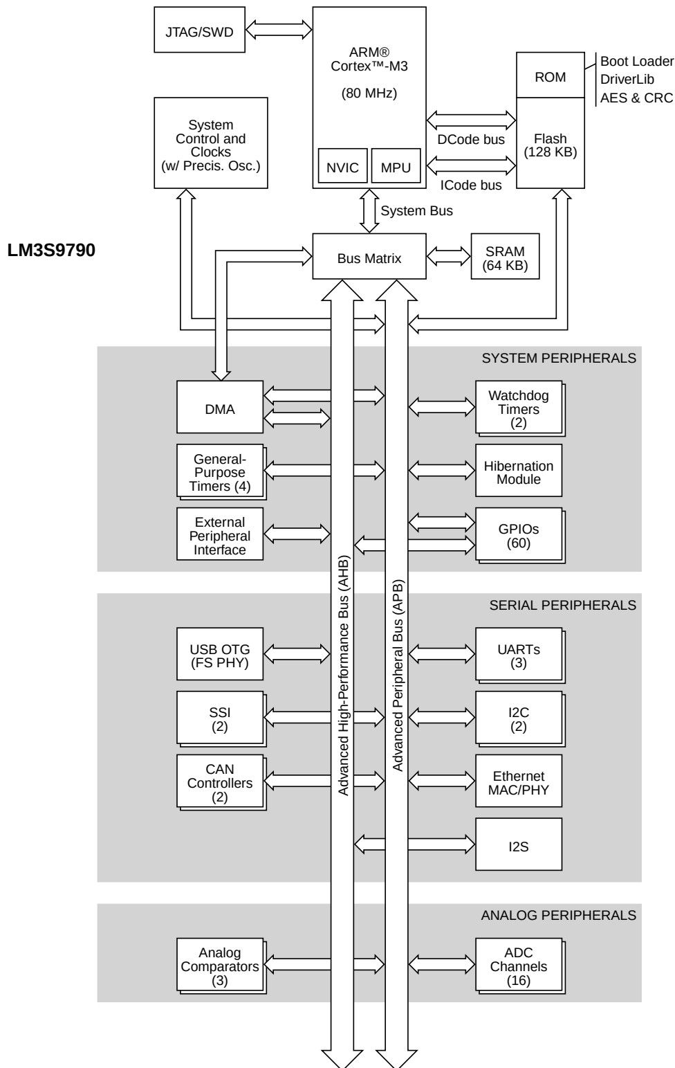
Figure 1-1. Stellaris LM3S9790 Microcontroller High-Level Block Diagram
