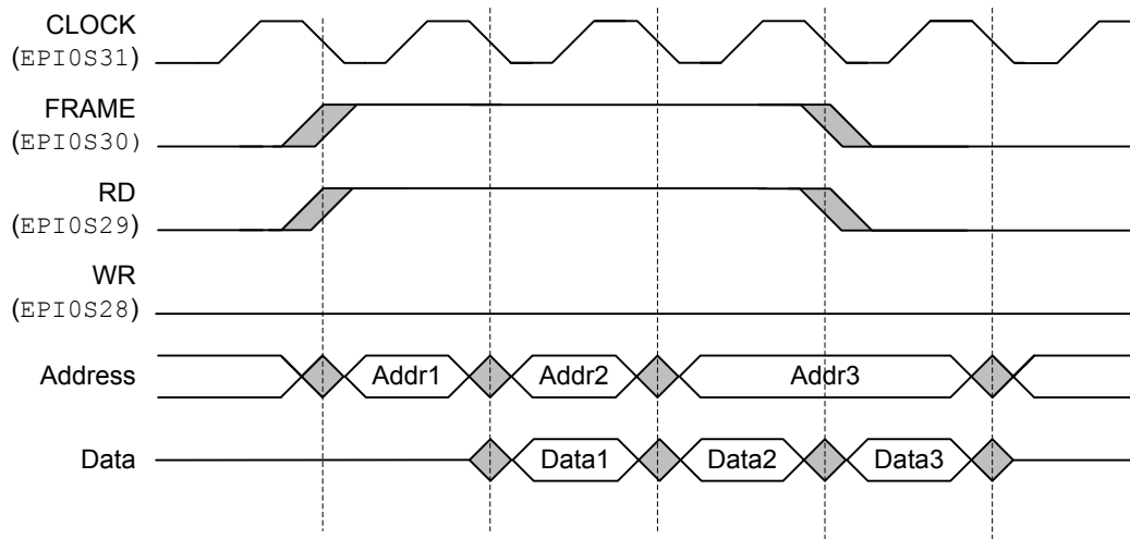
Figure 9-13. Read Accesses, FRM50=0, FRMCNT=0, RDCYC=1
