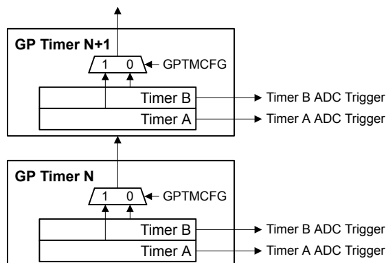
Figure 10-5. Timer Daisy Chain
