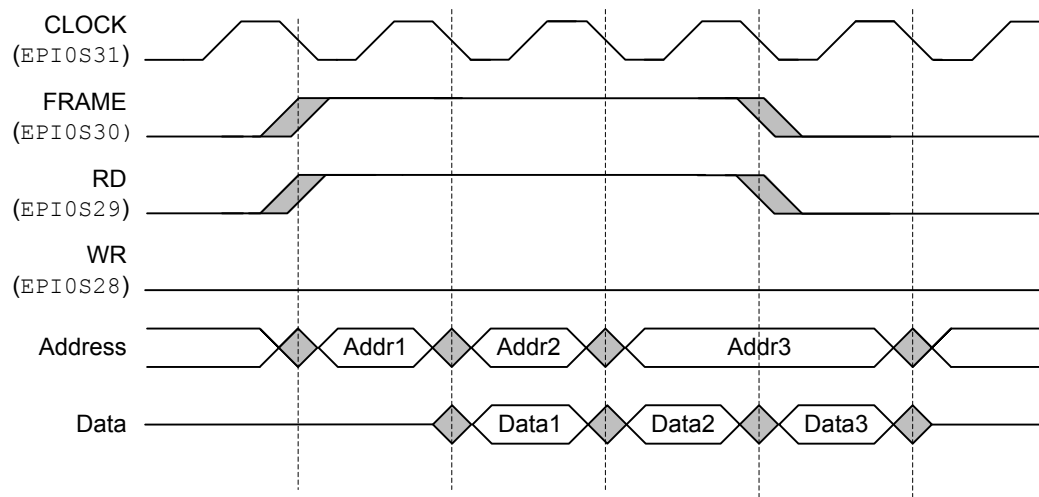
Figure 10-13. Read Accesses, FRM50=0, FRMCNT=0, RDCYC=1
