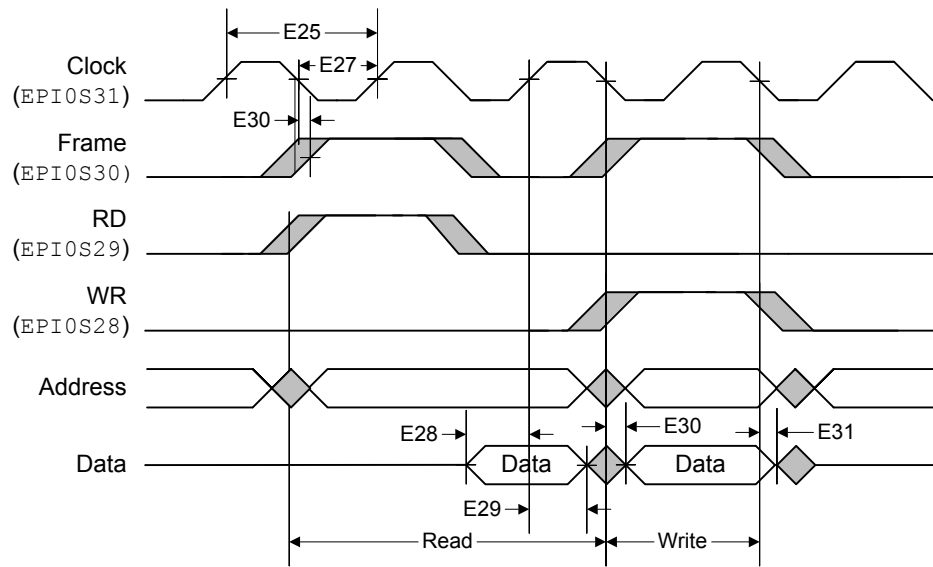
Figure 25-21. General-Purpose Mode Read and Write Timing
