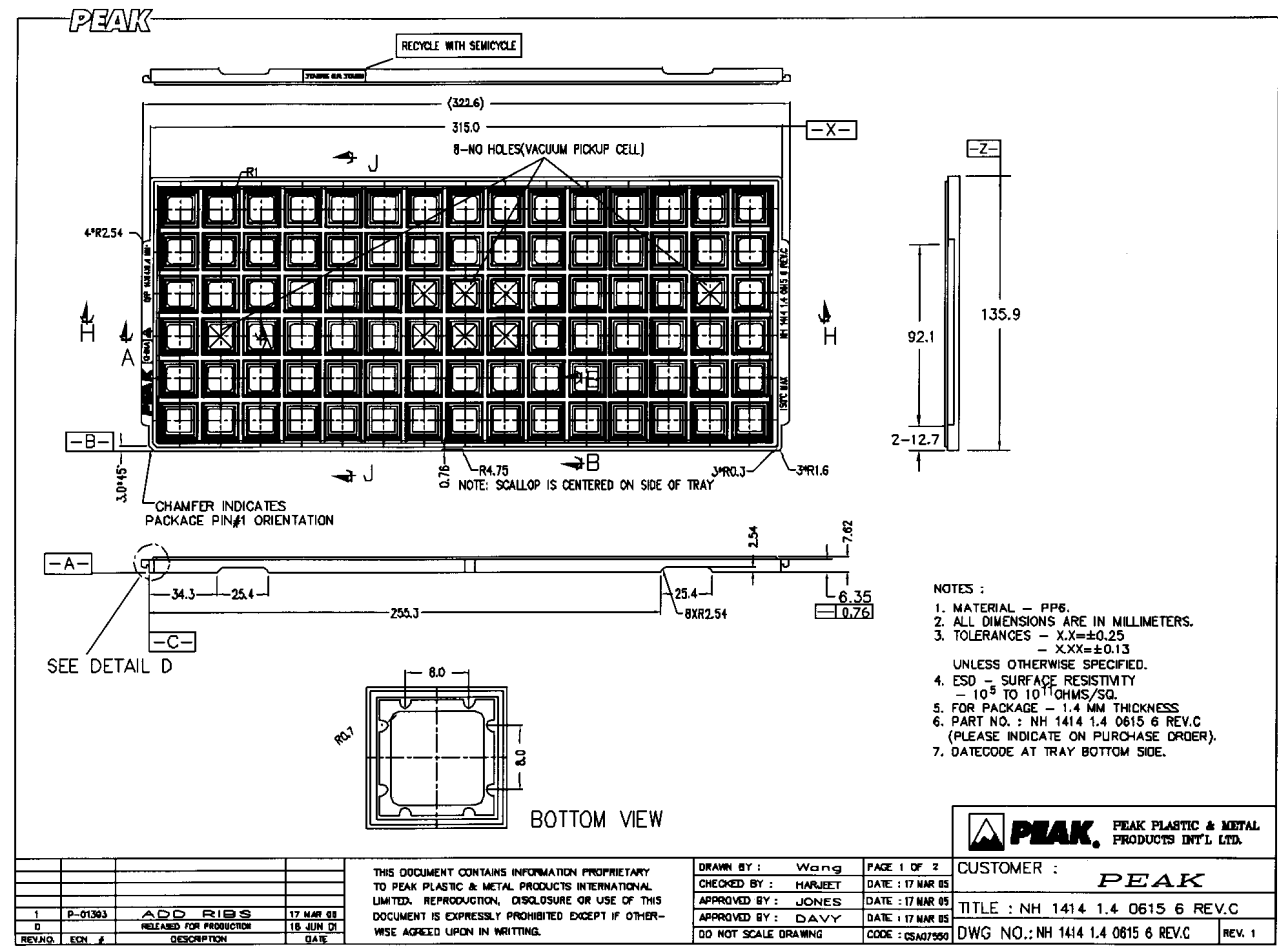
Figure C-2. 100-Pin LQFP Tray Dimensions
