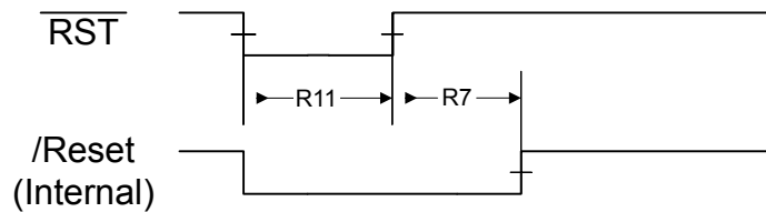
Figure 25-5. External Reset Timing ( \overline{RST} )
