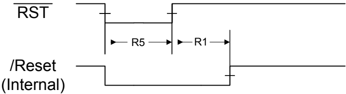
Figure 26-7. External Reset Timing ( \overline{\text{RST}} )
