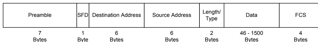
Figure 19-3. Ethernet Frame
