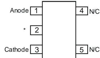
SC70-5**
