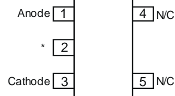
SC70-5**
