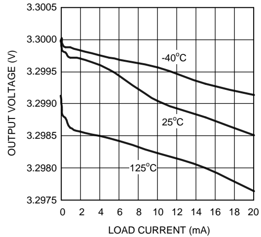
Figure 36. Load Regulation
