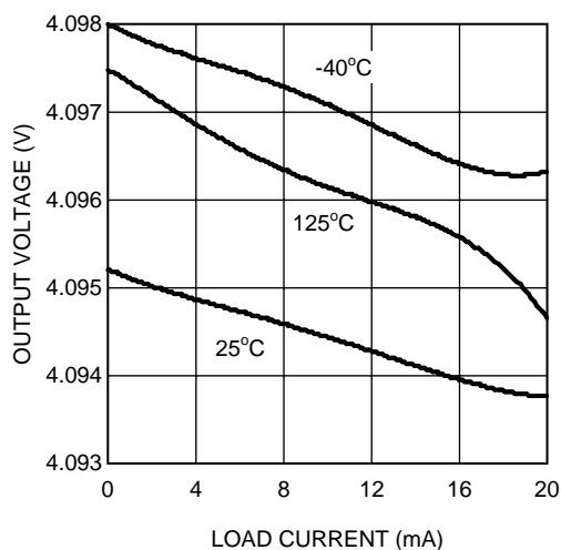
Figure 42. Load Regulation
