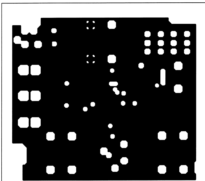
Figure 59. Recommended LQ PC Board Layout: Upper Inner-Layer Layout
