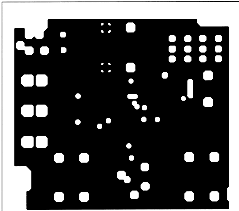
Figure 60. Recommended LQ PC Board Layout: Lower Inner-Layer Layout
