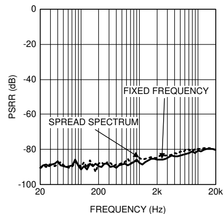
Figure 12. PSRR vs Frequency V_{DD} = 5\text{ V}, R_L = 8\ \Omega V_{\text{RIPPLE}} = 200\text{ mV}_{\text{PP}}, PV_1 = 7.8\text{ V}
