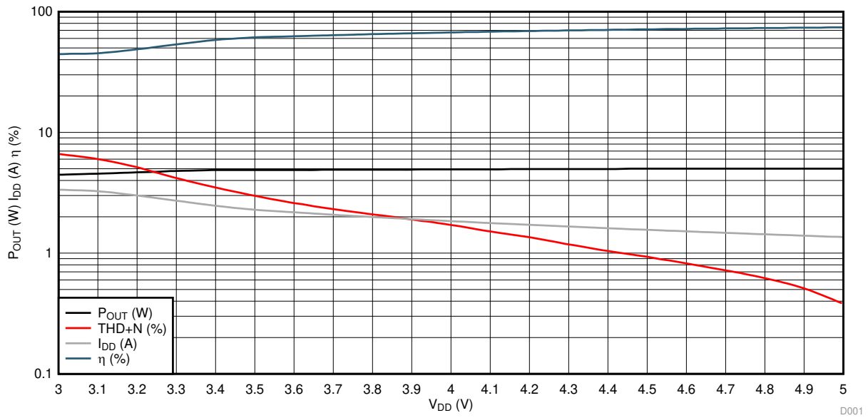
Figure 25. V_{DD} vs P_{OUT} , I_{DD} , and Efficiency With 4- \Omega Load
